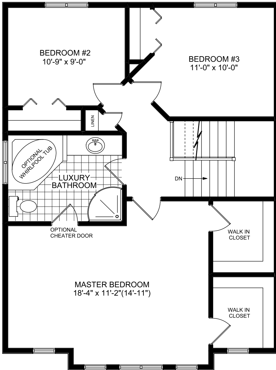
UPPER FLOOR PLAN 'B' 819 SQ.FT. THE RICHMOND
