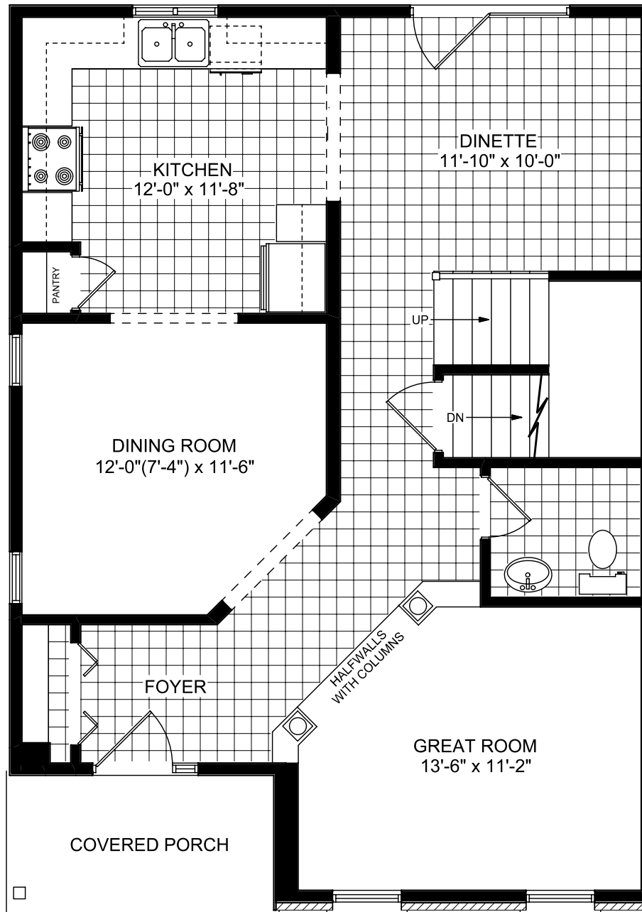
MAIN FLOOR PLAN 831 SQ.FT. THE RICHMOND
