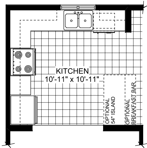
KITCHEN LAYOUT THE HAMPTON 'B'
