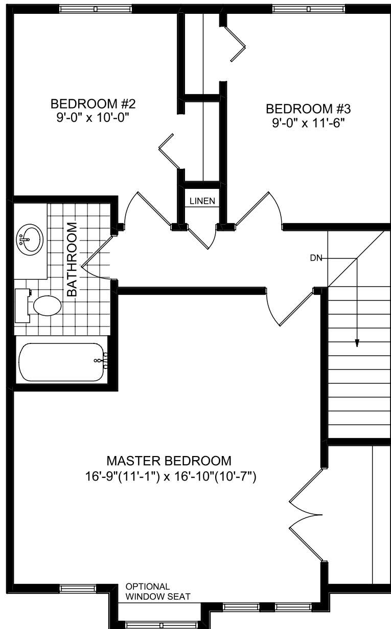
UPPER FLOOR PLAN 'A' 696 SQ.FT. THE HAMPTON
