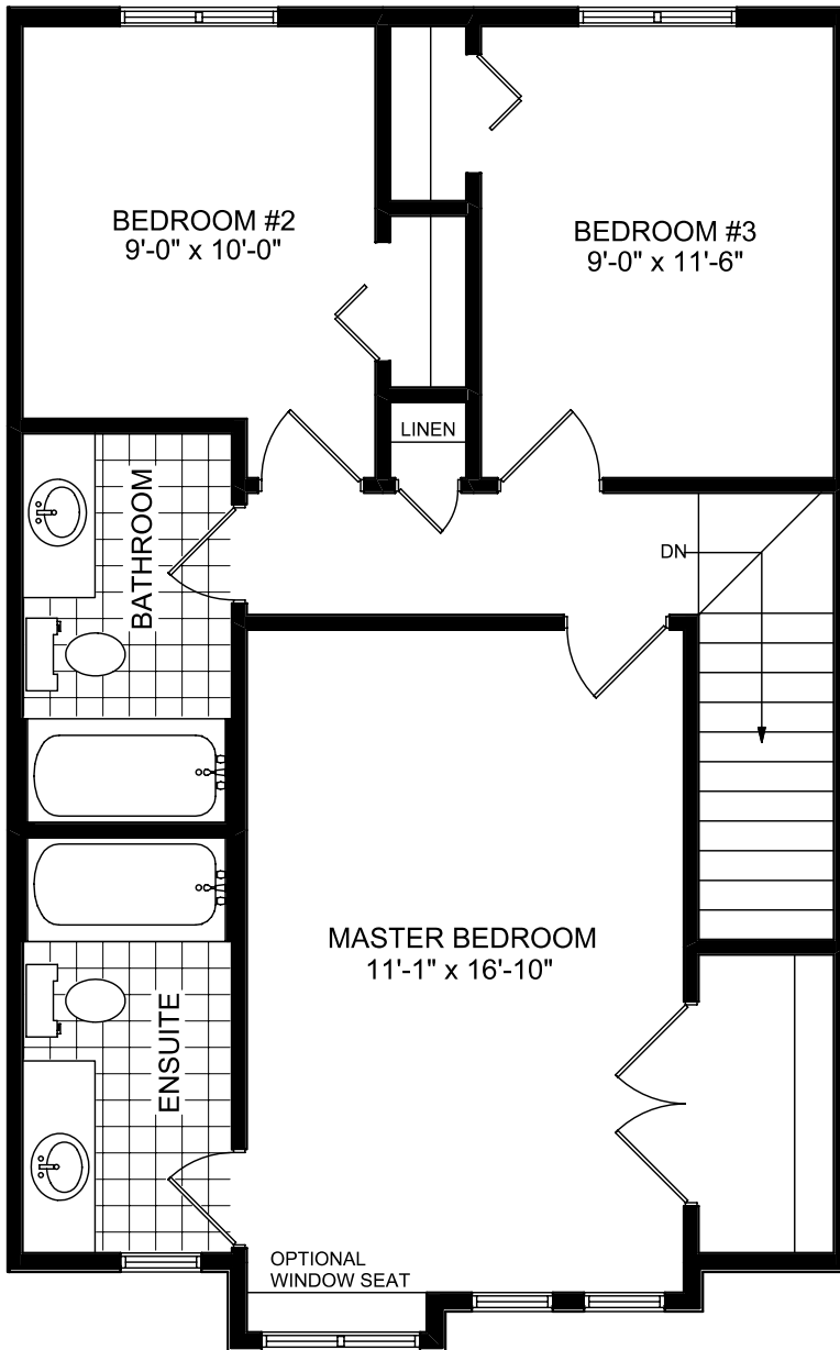
UPPER FLOOR PLAN 'B' 696 SQ.FT. THE HAMPTON
