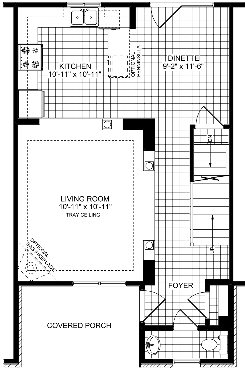
MAIN FLOOR PLAN 656 SQ.FT. THE HAMPTON 'A'
